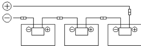
Series wiring
