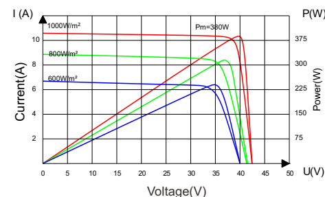
Current-Voltage&Power-Voltage Curve(380W)
